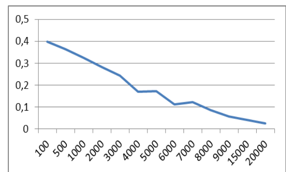
Fig. 6 – The training errors vs the amount of training cycles
